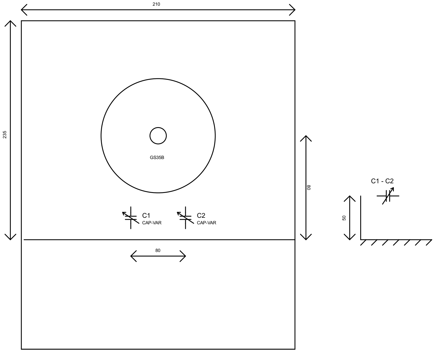
CATHODE-GRID CAVITY - DIMENSIONS
